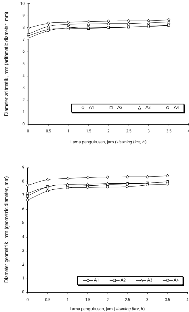
Gambar 6. Perubahan diameter geometrik dan aritmatik biji selama proses pengukusan. Figure 6. Geometric and arithmetic diameter changes during steaming process.
